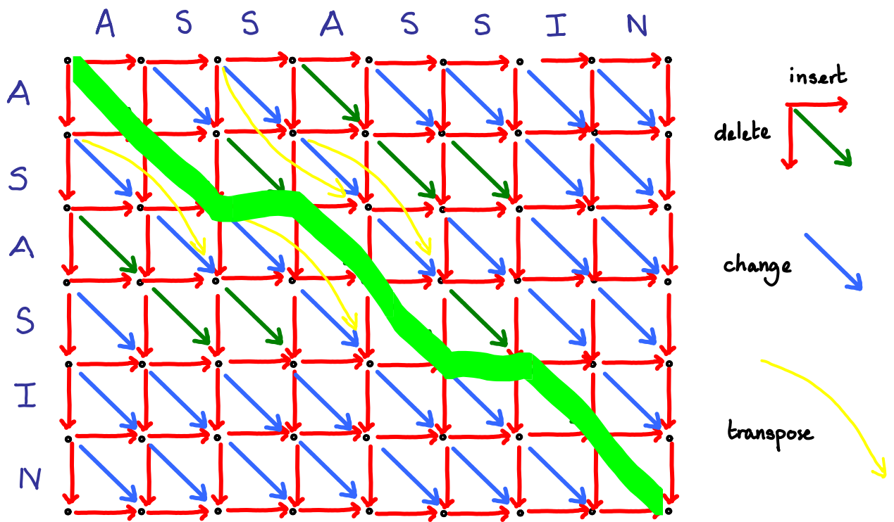
Shortest Path
